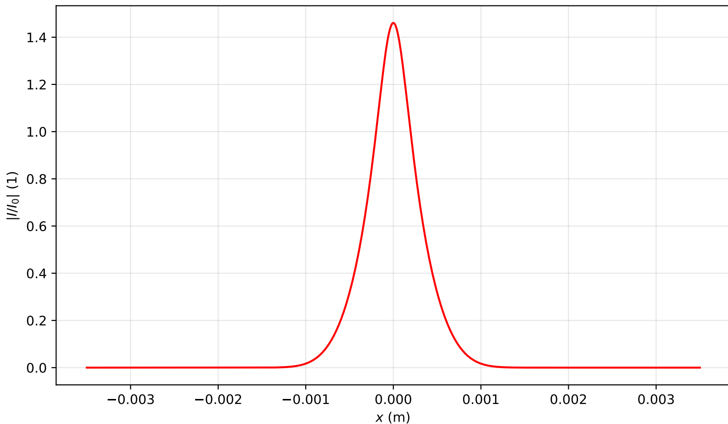
Intensity profile I(x, y = 0, z = 0.239)/I_0 , P_{in}=5.5P_{cr} , artificial time
